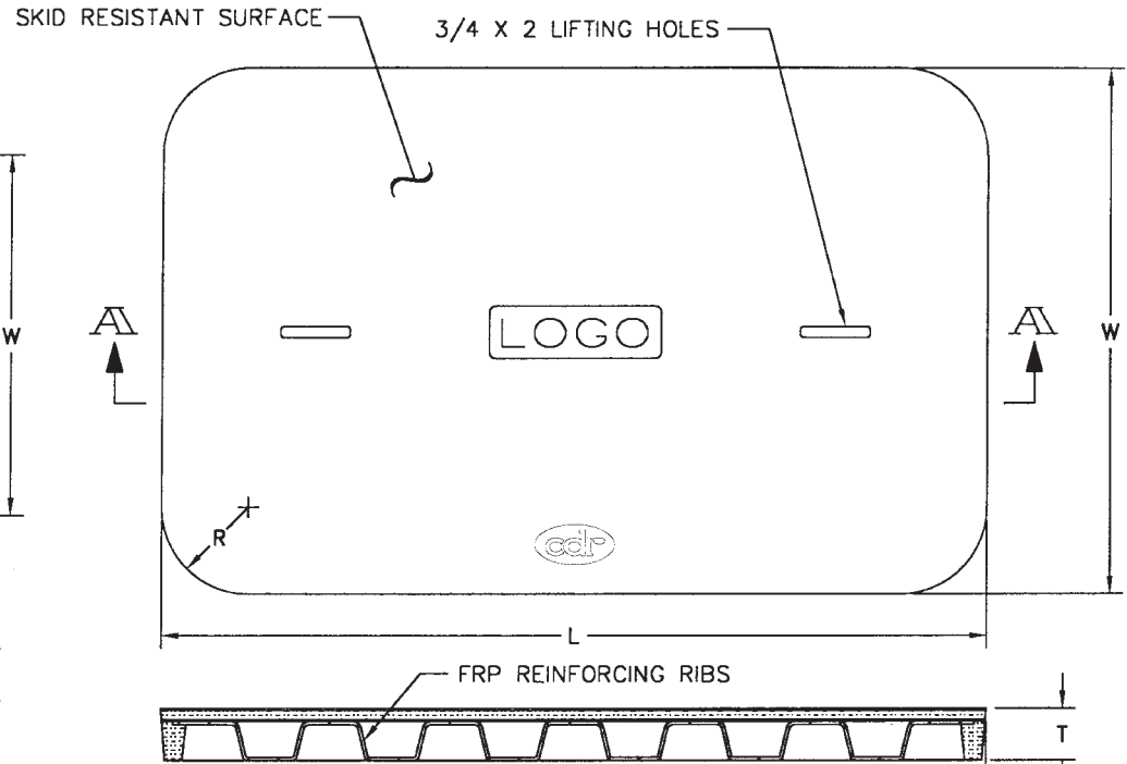
SECTION A - A STYLE 1
